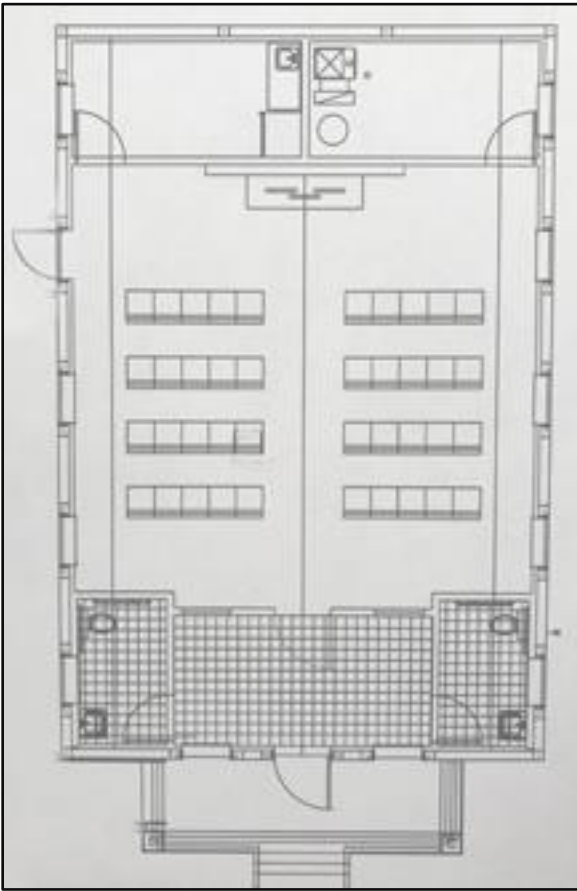
Floor Plan and Seating Layout For the New Life Chapel
